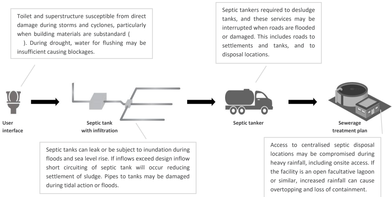
FIGURE 7: EXAMPLE OF CLIMATE-RELATED IMPACTS ALONG A SANITATION SERVICE DELIVERY CHAIN (SERVICED SEPTIC TANK)
